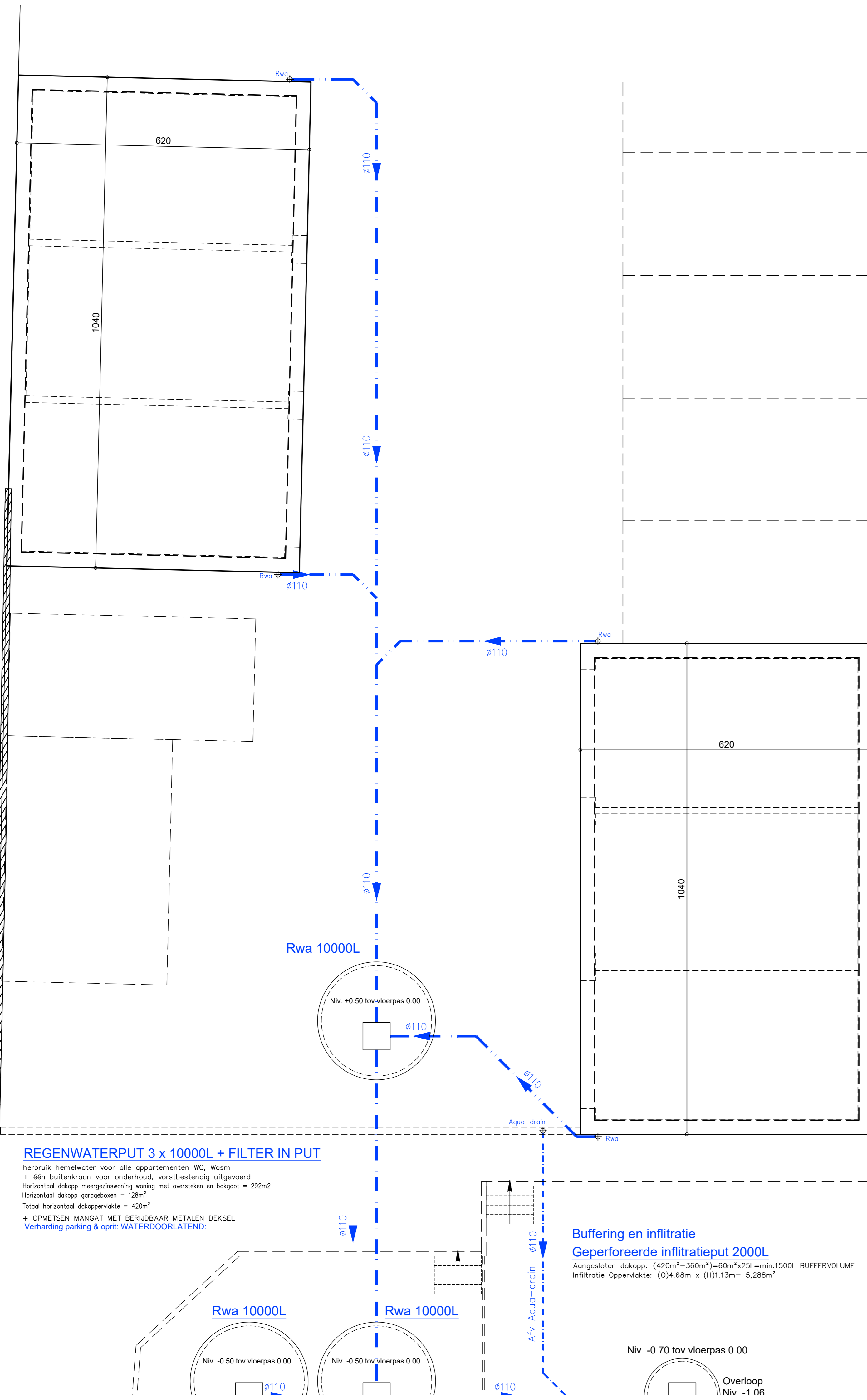
PLAN FUNDERINGEN & RIOLERINGEN GARAGES
